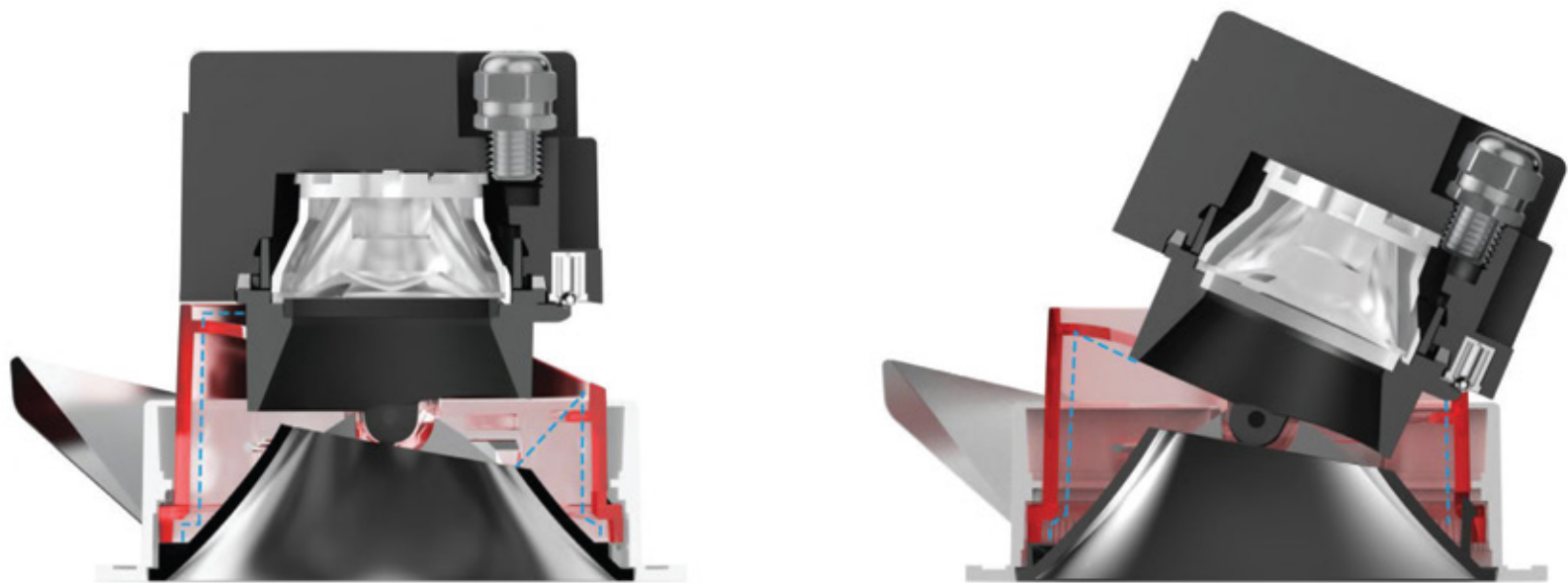
Note: The red part is the adjustment middle ring, and light leakage prevention design show in the schematic diagram
